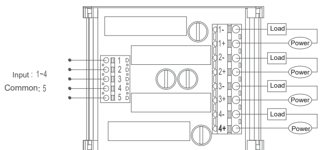
DRA-4A/K-KSF /KSL Series Wiring Diagram
