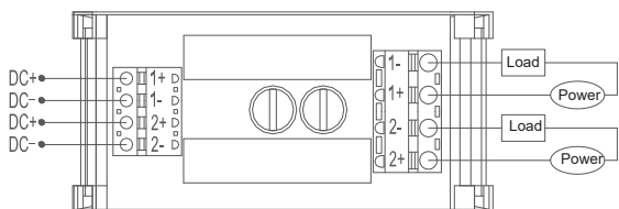
DRA-2-KSF/ KSL Series Wiring Diagram
