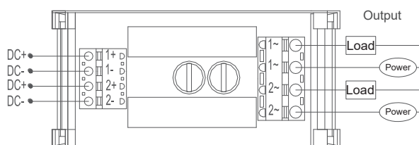
DRA-2-KSD Series Wiring Diagram
