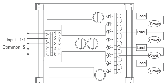
DRA-4A/K-KSD Series Wiring Diagram
