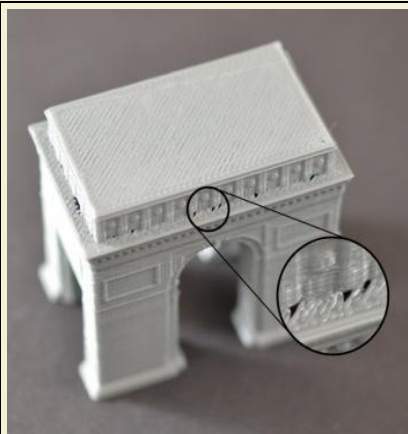
Gaps in Floor Corners
