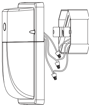
1. Connect Wires
