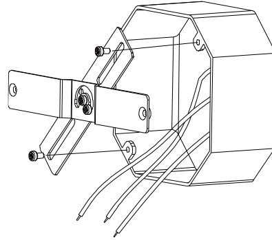
1. Installation back plate to junction box
