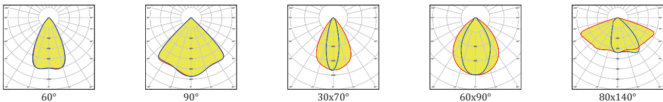
Rectangular beam, meet the channel lighting requirement
