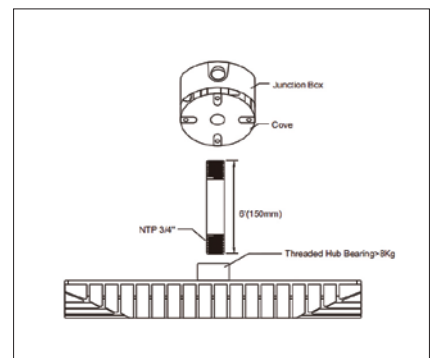
3/4" Pole Pedant
