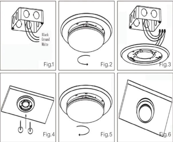
COMPATIBLE WITH 2.75/3.5/4 INCH JUNCTION BOX
